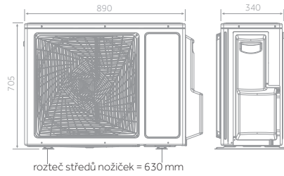
1U125
