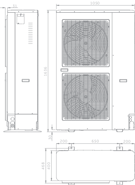
1UH200 / 1UH250
